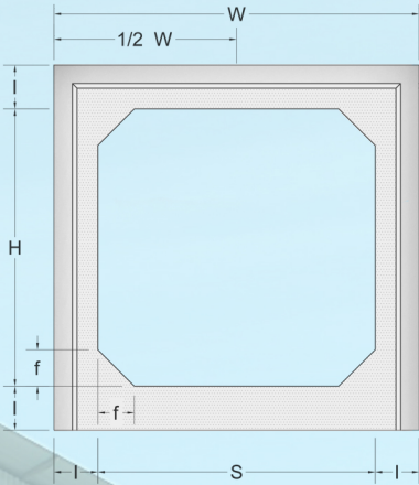
Box Culvert
